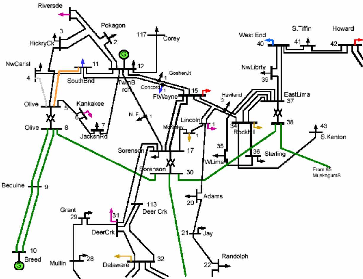
Fig. 2. Initial effect of the outage of line 4-5 in the 118-bus test system.
